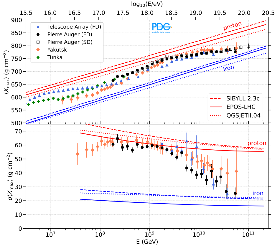
Figure 30.8: Measurements of \langle X_{\max} \rangle (top) and \sigma(X_{\max}) (bottom) obtained by the Telescope Array [141, 142], Pierre Auger Observatory [143, 144], Yakutsk [125] and Tunka [145] UHECR detectors, compared to predictions for proton and iron nuclei using the hadronic models SIBYLL2.3c [146], EPOS-LHC [120] and QGSJET-II.04 [119]. Detection techniques: fluorescence (FD), Cherenkov (Yakutsk, Tunka, and TA below \simeq 1 EeV), and using the surface detector array of the Auger Observatory (SD). For a compilation including experiments using the radio technique see [140].
