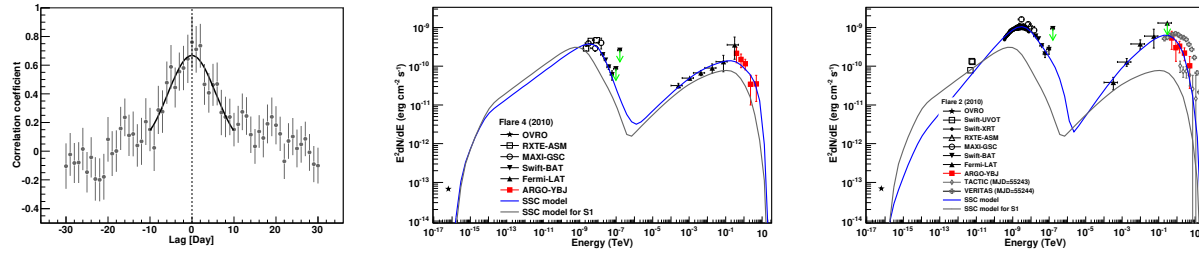
Figure 30.11: The multi wavelength analysis of Mrk 421 involving measurements over wide energy range from radio to TeV \gamma -ray during 4.5 years when ARGO-YBJ and LAT were operated [221]. The discrete correlation function between the light curves in X-ray band and TeV \gamma -ray band is calculated and clearly shows no time lag between emissions in the two bands [221] (left panel). The SED significantly changes from steady states (grey solid lines in middle and right panels) to flaring states depending on the strength of flares. Comparing a small flare in the middle panel and a larger one in right panel, the later has harder SED in VHE band. [221].
