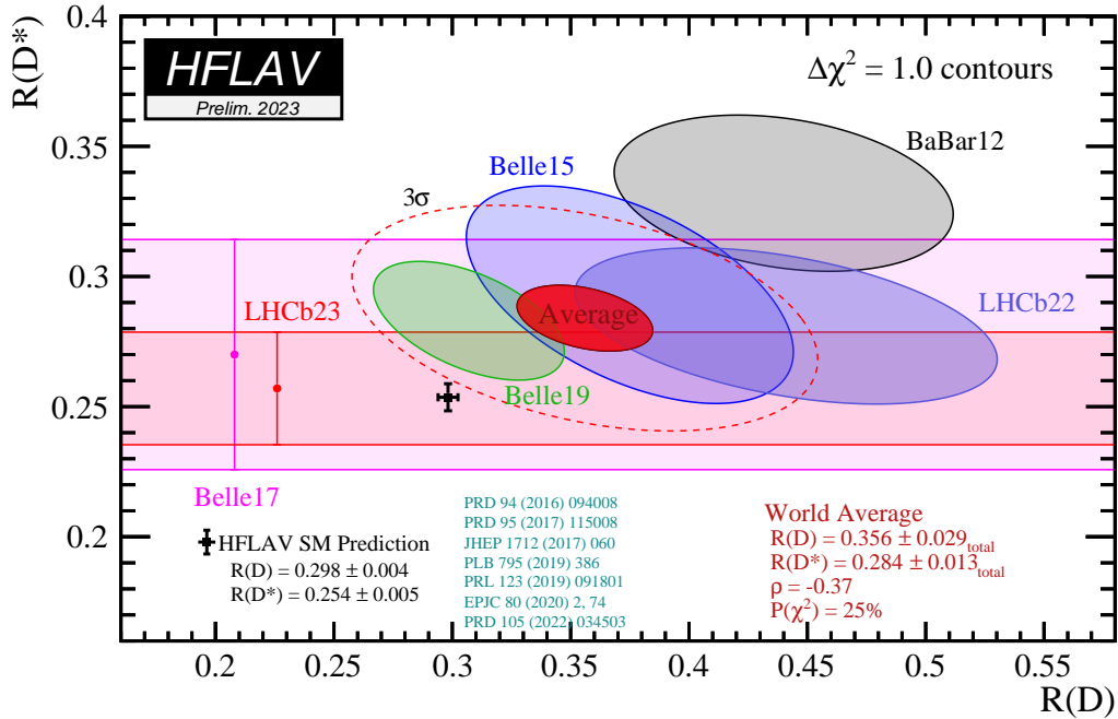
Figure 76.2: Measurements of R(D) and R(D^*) and their two-dimensional average compared with the average predictions for R(D) and R(D^*) given in Eq. 76.62. Contours correspond to \Delta\chi^2 = 1 i.e. , 68% CL for the bands and 39% CL for the ellipses. The experiment-lattice QCD-HQET predictions and the experimental average deviate from each other by 3.3\sigma . The dashed ellipse corresponds to a 3\sigma contour of the experiment average (99.73% CL).
