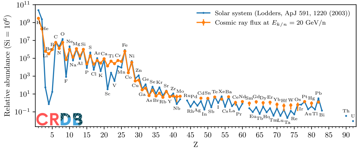
Figure 30.2: CR abundances compared with solar system ones [67]. Modified from [38].
