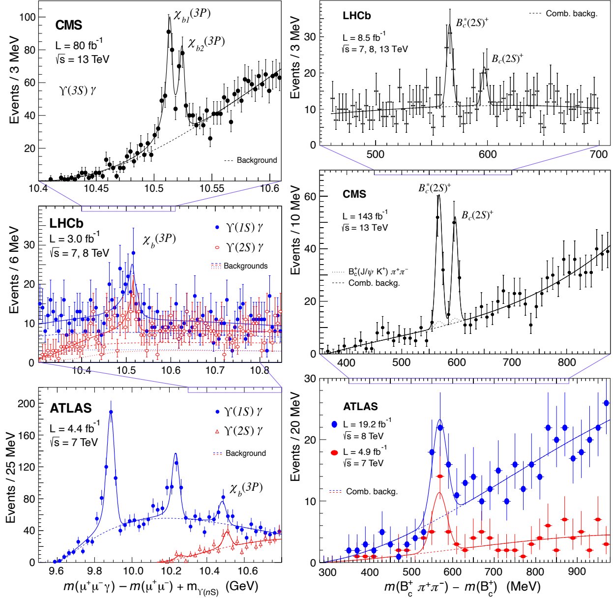
Figure 77.2: (Left Column) Invariant mass distributions measured by the ATLAS [29] (bottom), LHCb [31] (middle) and CMS [32] (top) experiments in their searches for the \chi_b(3P) states through their radiative decays to one of the S-wave bottomonia. (Right Column) Invariant mass distributions measured by the ATLAS [33] (bottom), CMS [34] (middle) and LHCb [35] (top) experiments in their searches for B_c^\pm excited states decaying to the B_c^\pm ground state with the emission of two charged pions.
