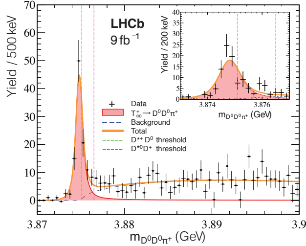
Figure 77.6: The D^0D^0\pi^+ invariant mass distribution from LHCb [109, 110].
