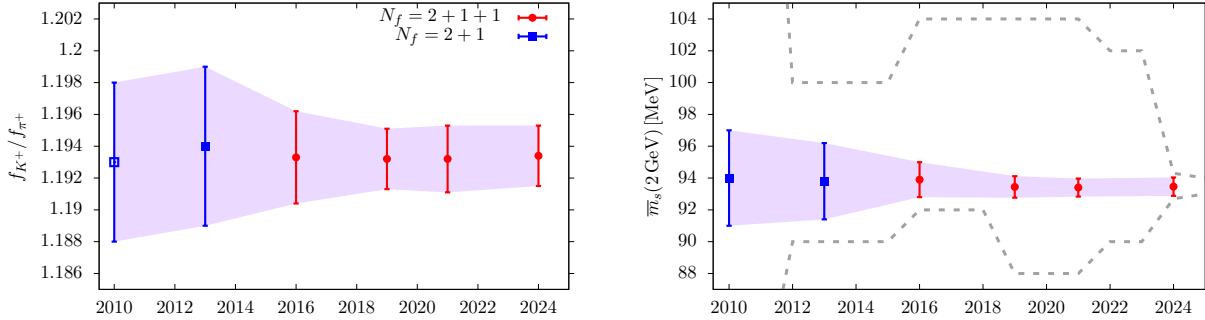
Figure 17.3: History of the FLAG averages of LQCD results for the ratio of kaon and pion decay constants f_{K^+}/f_{\pi^+} and the strange-quark mass \bar{m}_s(2 \text{ GeV}) (defined in the \overline{MS} scheme, \mu = 2 \text{ GeV} ) [60, 85, 192–195]. In both cases we see a large improvement in the uncertainty over the 14-year timespan—by a factor of 2.5 for f_{K^+}^+/f_{\pi^+}^+ (the 2010 result is for the isospin-symmetric f_K/f_\pi ) and a factor of 5 for m_s —as ensemble sizes have grown for improved statistical errors and lattice spacings have become finer and light quark masses closer to the physical point for improved systematic errors. There has also been a shift from n_f = 2+1 to n_f = 2+1+1 simulations over time. The grey dashed lines for \bar{m}_s indicate the \pm 1\sigma band given in the PDG particle listings (pdglive for 2025). The PDG’s evaluation of \bar{m}_s is now in good agreement with the average of the lattice QCD results.
