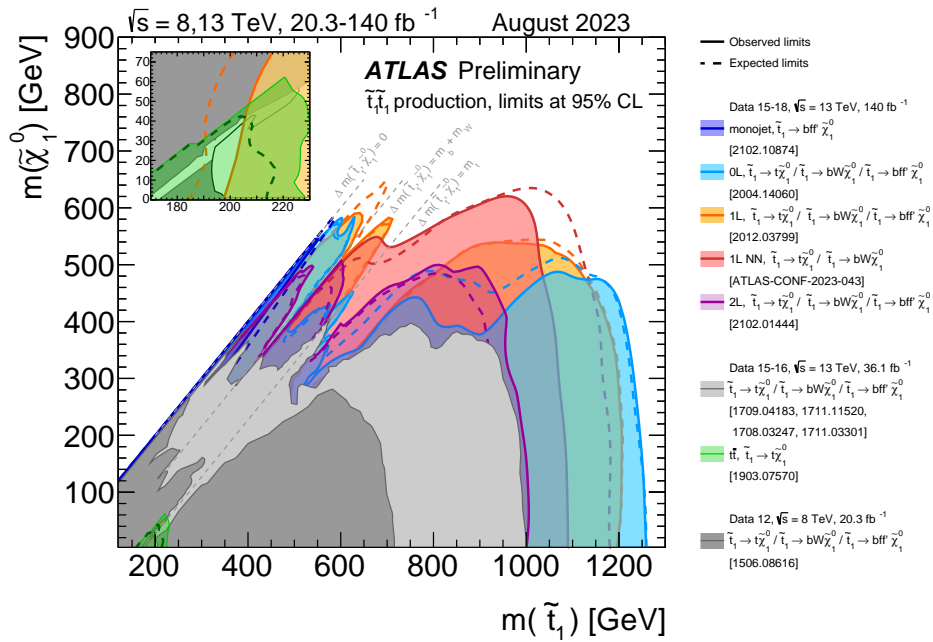
Figure 88.6: A summary of the 95% C.L. exclusion contours in the stop-neutralino mass plane for various possible decay chains, including two-, three- and four-body decays, as obtained in dedicated analyses by ATLAS.
