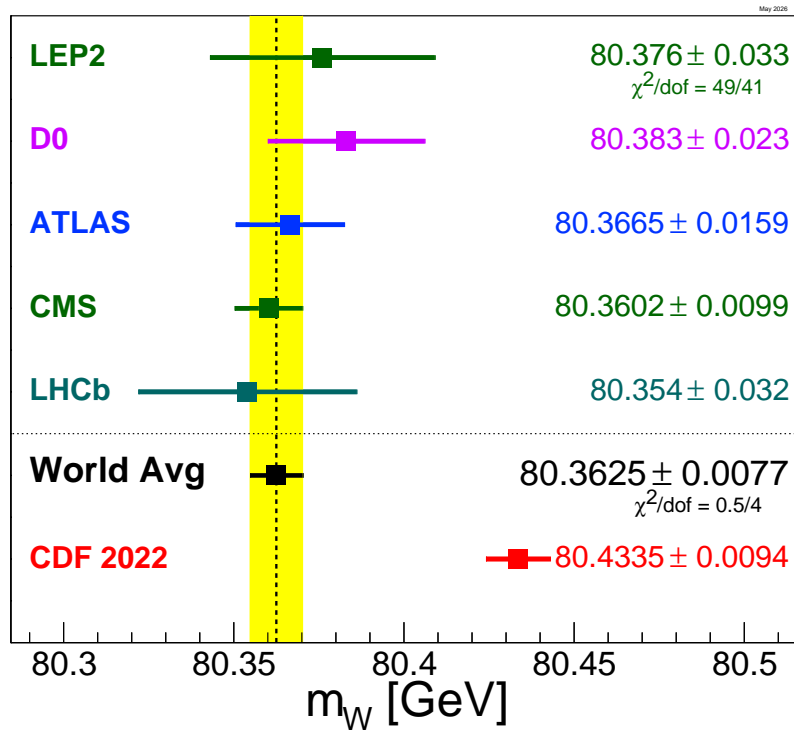
Figure 54.1: Measurements of the W -boson mass by the LEP, Tevatron and LHC experiments as well as their combination. Below the combination, the CDF 2022 result is shown which is currently not used in the world average.
