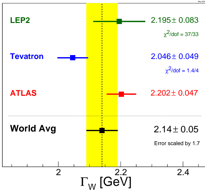
Figure 54.2: Measurements of the W -boson width by the LEP, Tevatron and LHC experiments.
